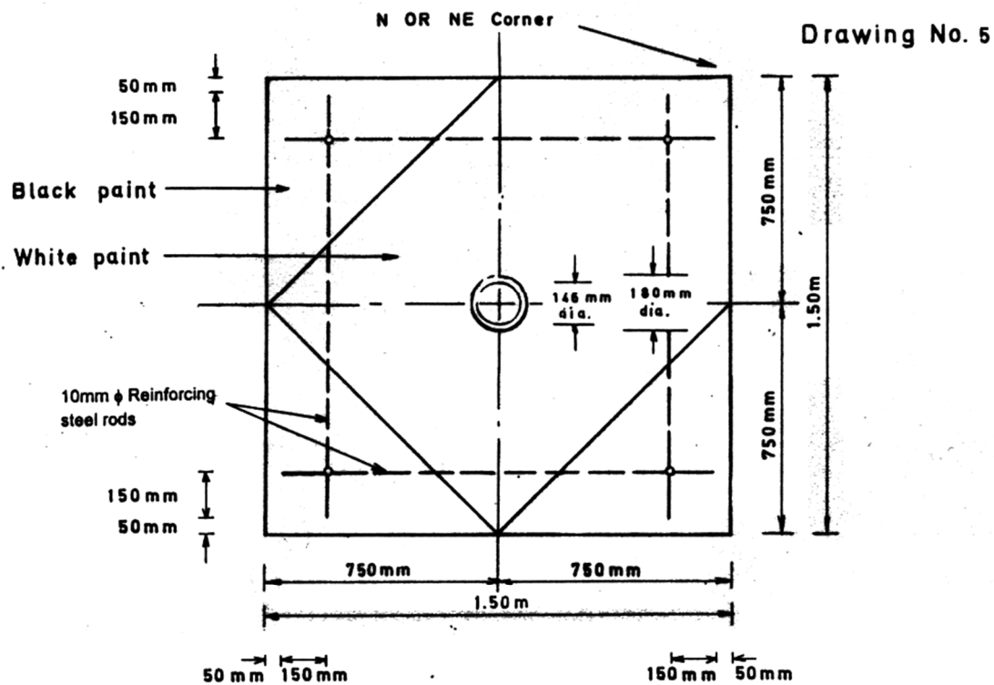
PLAN VIEW
